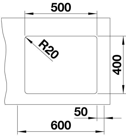
Cut-out
